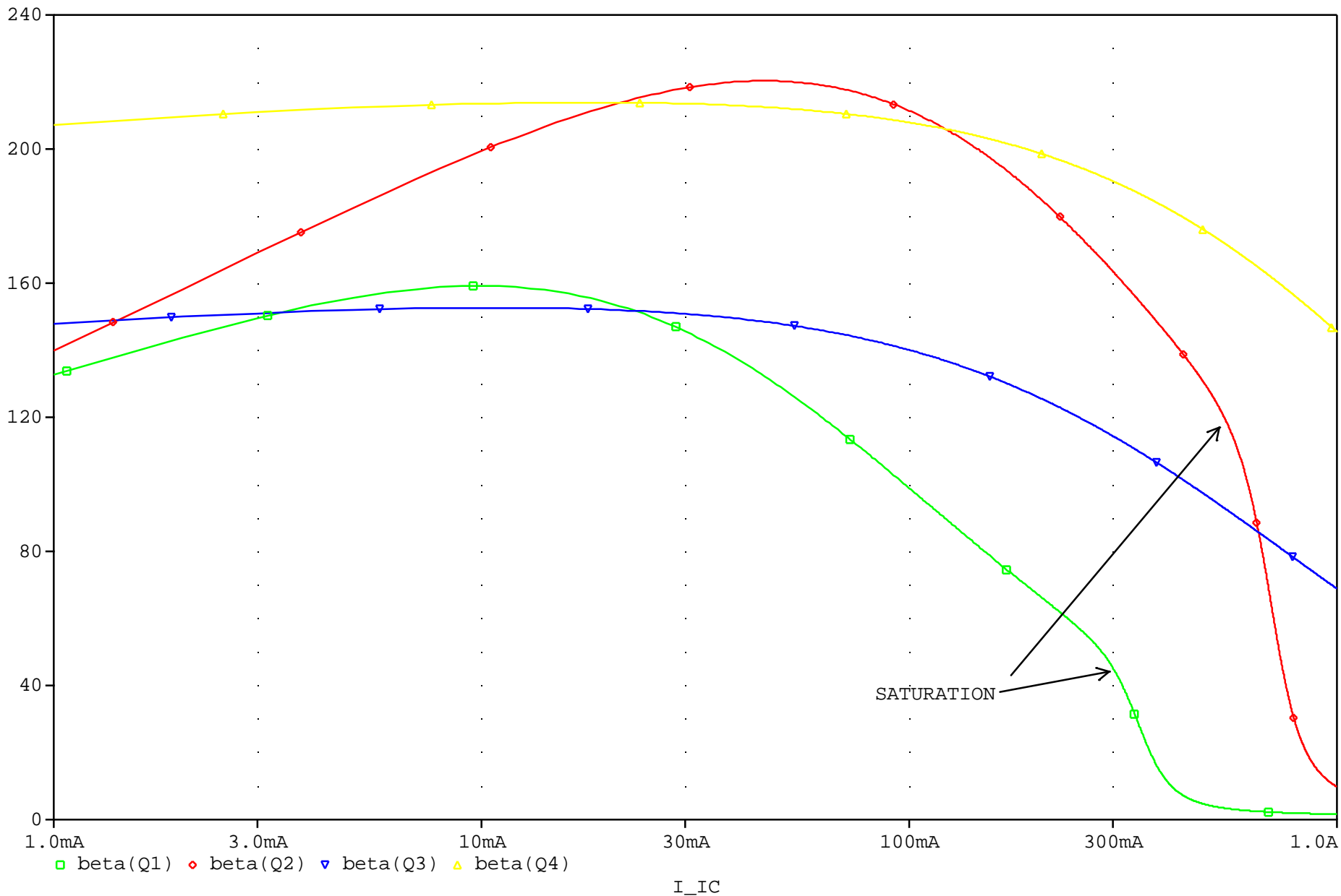
Beta Curves...VCE = 0.5V
