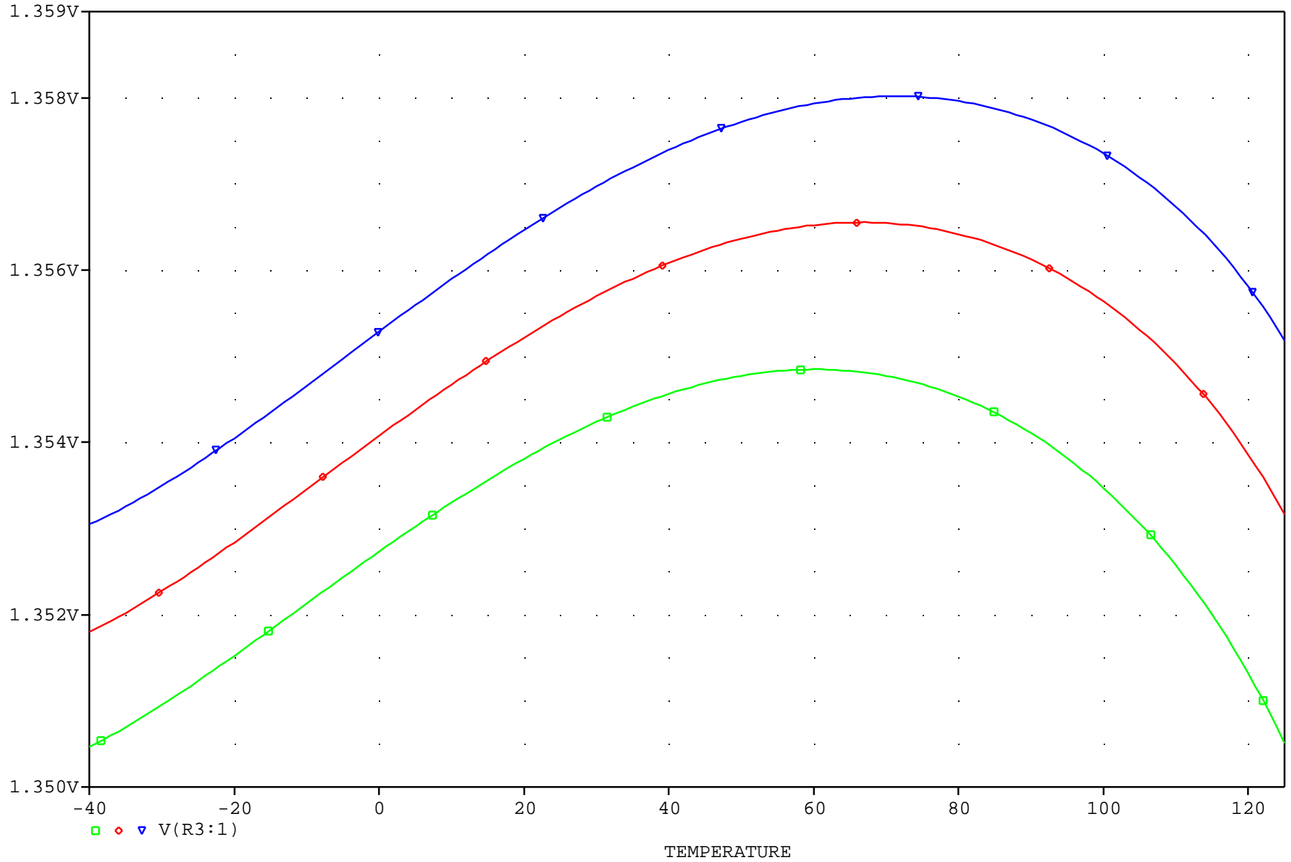
CA3046 BandGap versus Temperature and V1 = 4.5V, 5.0V, 5.5V
