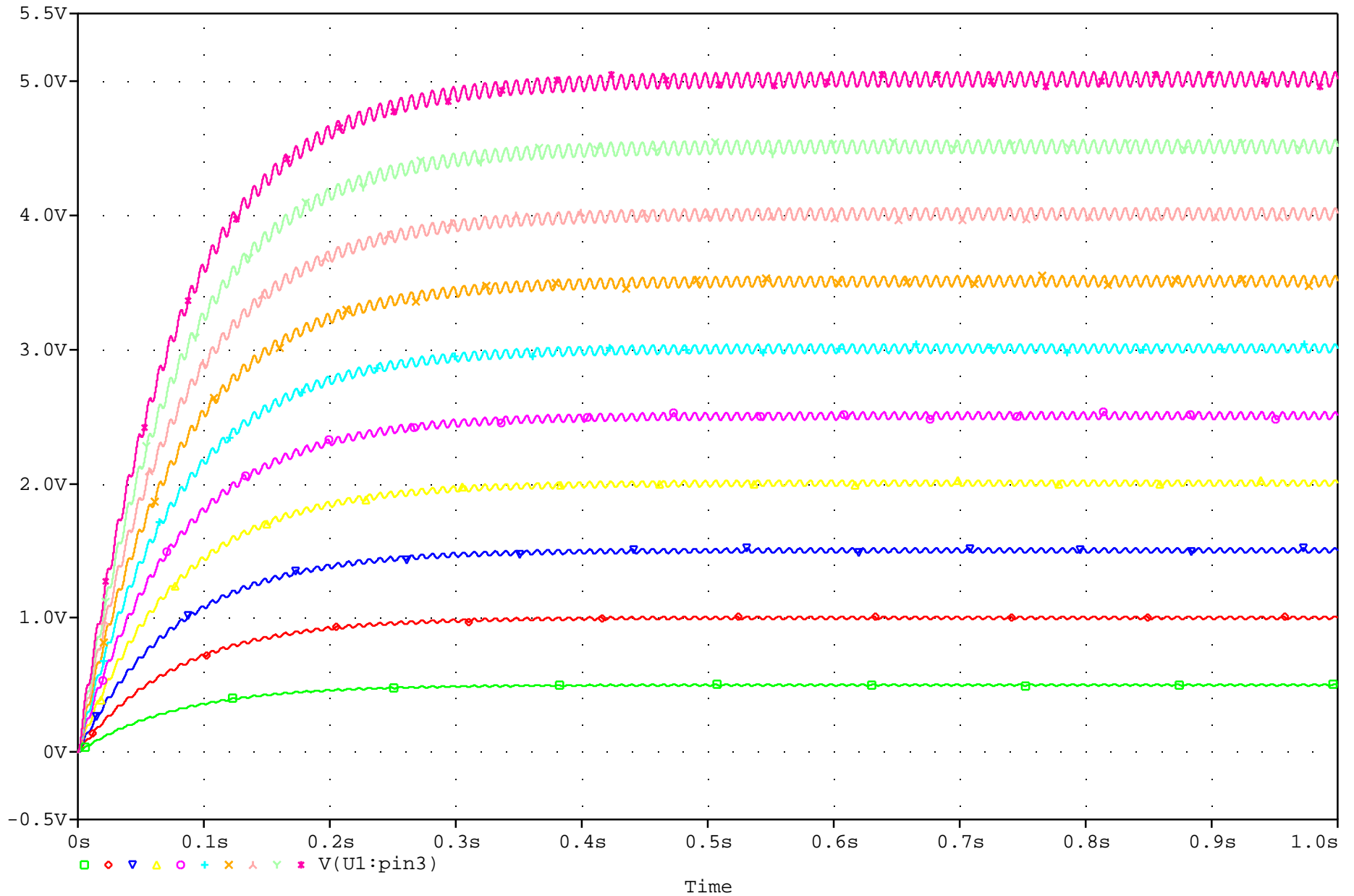
Current Transformer Rectified ("IP" Stepped from 1mA to 10mA in 1mA Steps)
