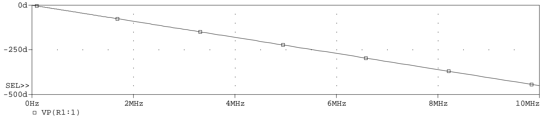
(A) Delay=ExcessPhase (50-ohm T-Line with 125ns Delay)
