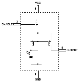
Block Diagram
