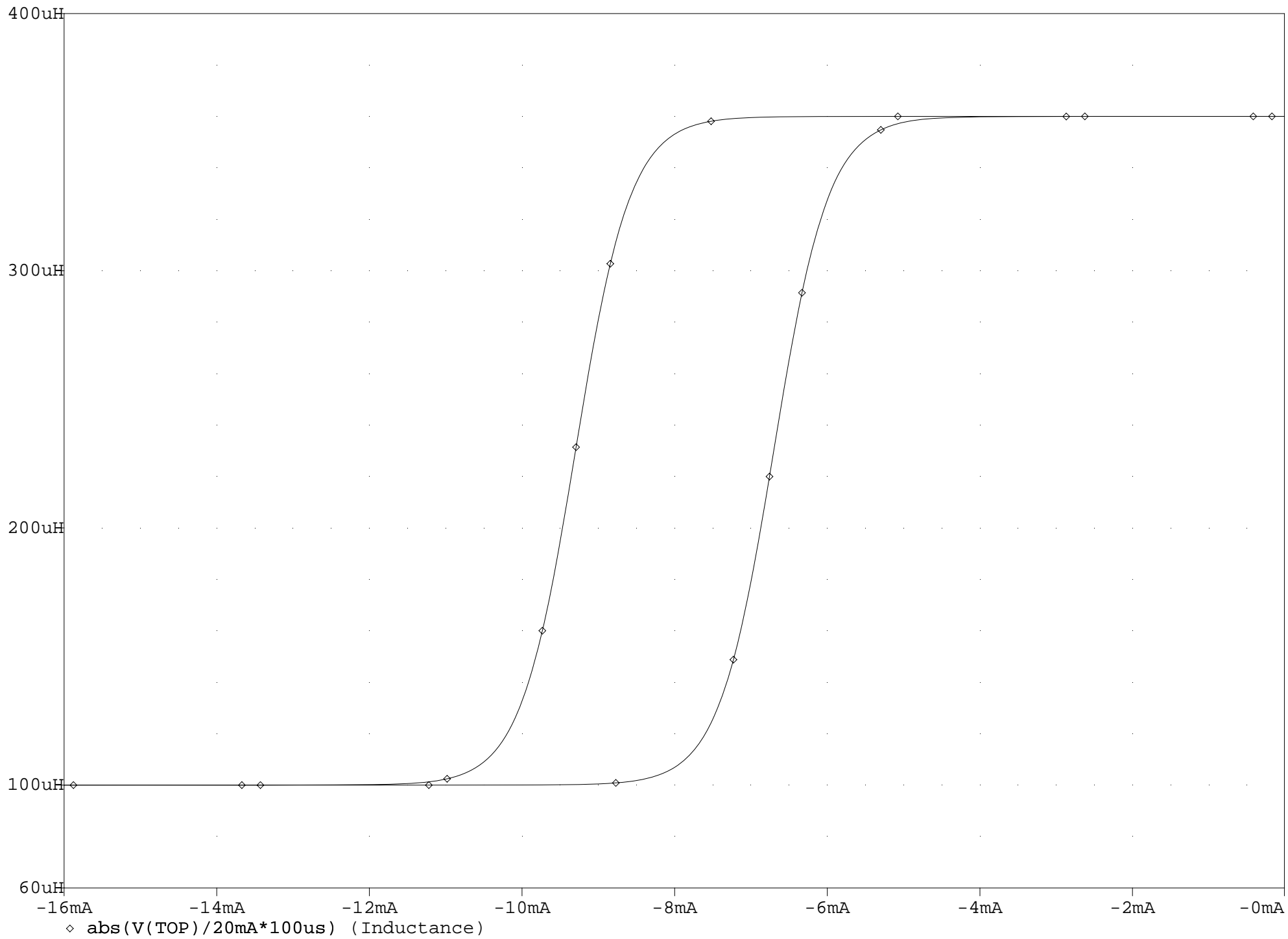
(A) Field Sensor Spice Model with Hysteresis Added
