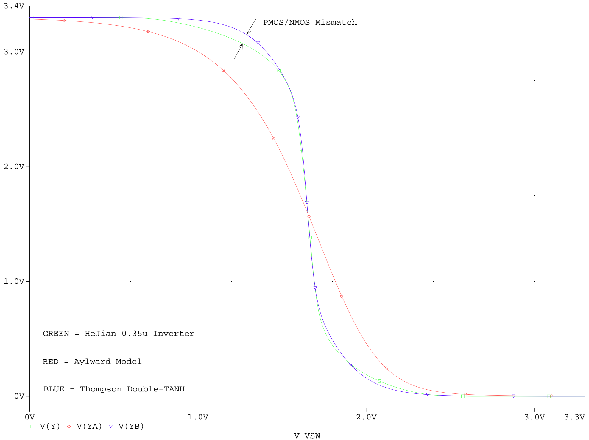
Two Spice Behavioral Models Compared to Real HeJian 0.35u Inverter
