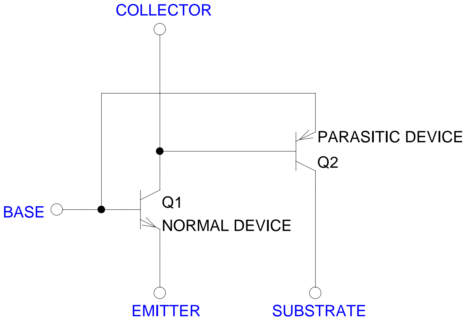
NPN with PARASITIC PNP
