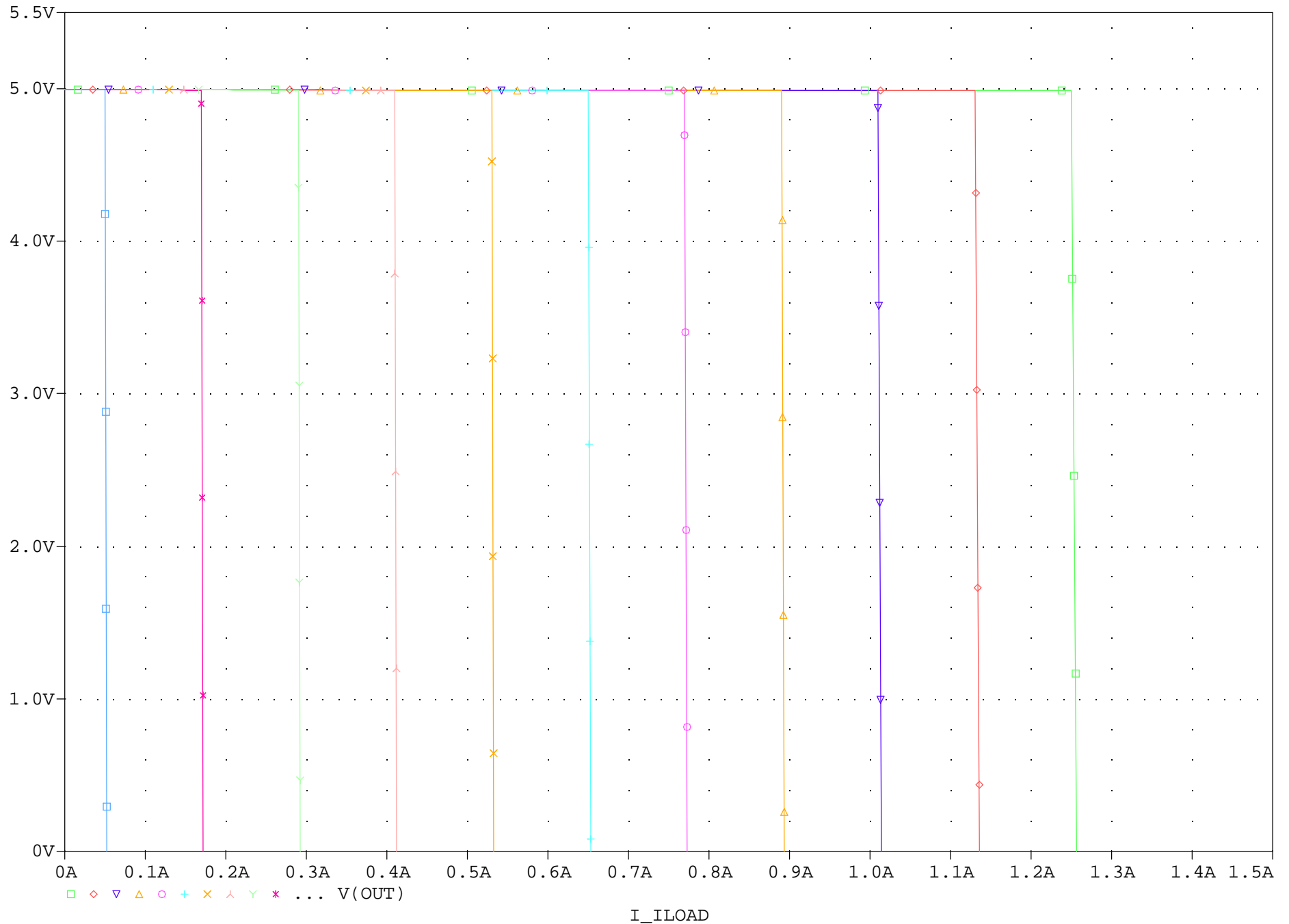
Simple Regulator with Adjustable Current Limit (SED), ILIM 0 -> 6mA in 0.5mA Steps
